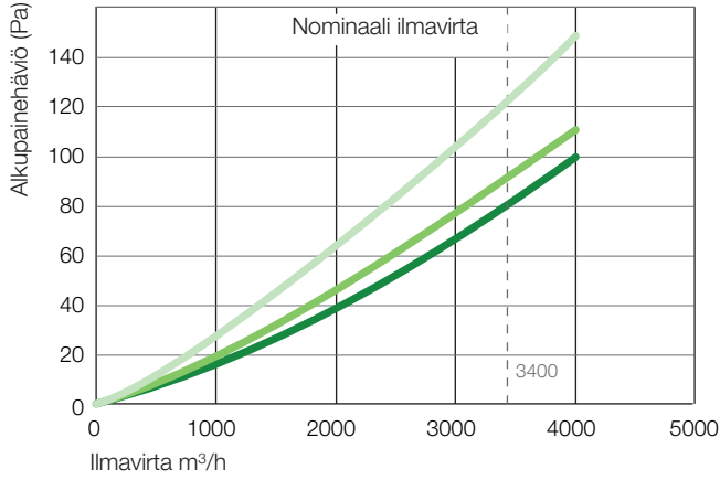
DriPak GX - ePM1 55% 592x592x360/8 pussia / ePM1 55% 592x592x525/8 pussia / ePM1 55% 592x592x635/8 pussia
