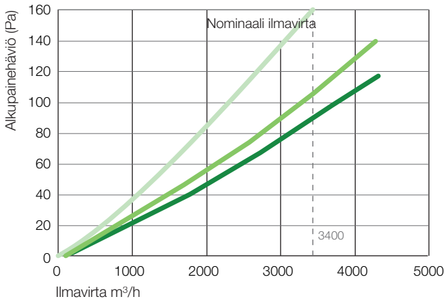
DriPak GX - ePM1 60% 592x592x360/8 pussia / ePM1 60% 592x592x525/8 pussia / ePM1 60% 592x592x635/8 pussia
