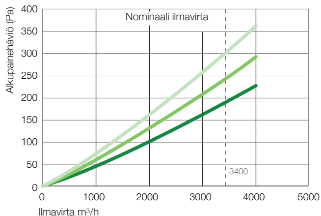
DriPak GX - ePM1 90% 592x592x360/8 pussia / ePM1 90% 592x592x525/8 pussia / ePM1 90% 592x592x635/8 pussia
