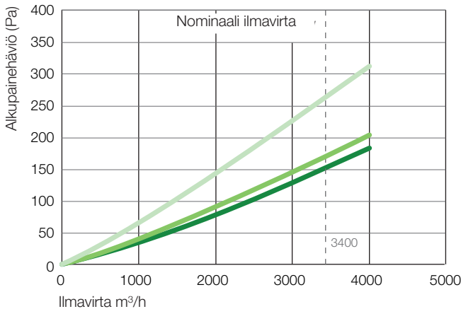
DriPak GX - ePM1 85% 592x592x360/8 pussia / ePM1 85% 592x592x525/8 pussia / ePM1 85% 592x592x635/8 pussia
