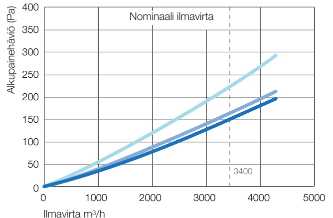
DriPak GX - ePM1 85% 592x592x360/10 pussia / ePM1 85% 592x592x525/10 pussia / ePM1 85% 592x592x635/10 pussia
