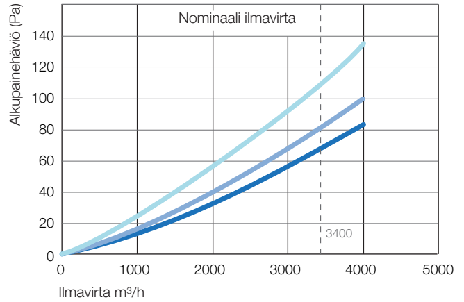
DriPak GX - ePM1 55% 592x592x360/10 pussia / ePM1 55% 592x592x525/10 pussia / ePM1 55% 592x592x635/10 pussia
