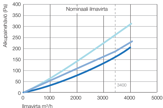
DriPak GX - ePM1 90% 592x592x360/10 pussia / ePM1 90% 592x592x525 10 pussia / ePM1 90% 592x592x635/10 pussia
