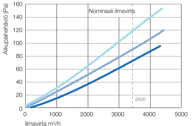
DriPak GX - ePM1 60% 592x592x360/10 pussia / ePM1 60% 592x592x525/10 pussia / ePM1 60% 592x592x635/10 pussia
